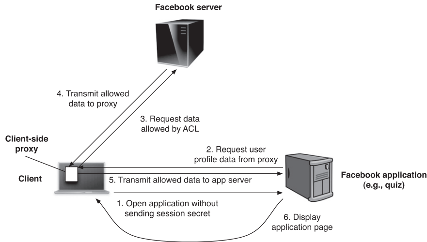
Fig. 2. Modified data-flow with PoX.
