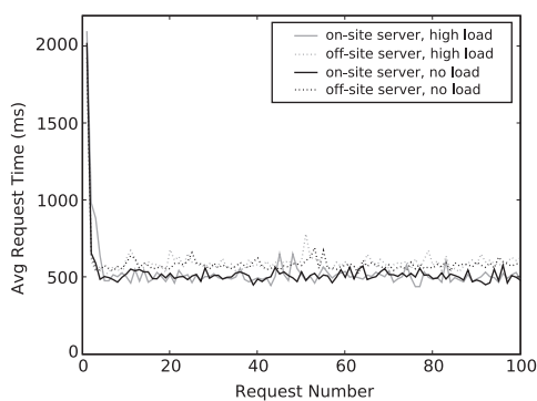
(a) Request times for high / low load
