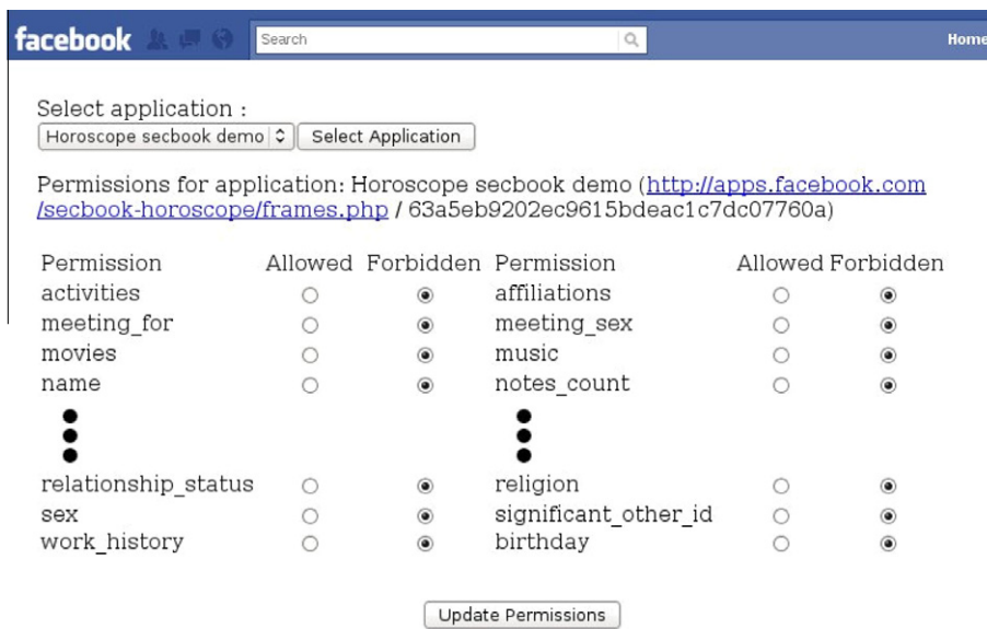
Fig. 4. Managing ACLs with PoX.
