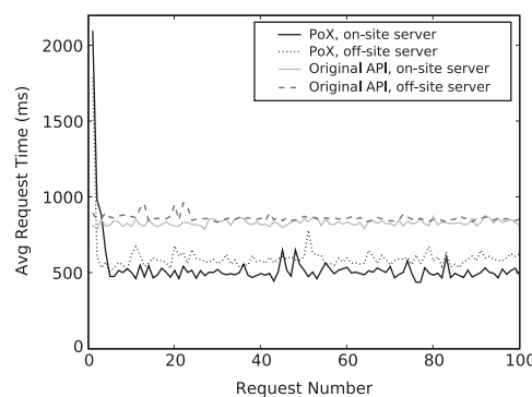
(b) Request times for PoX and the original FB API
