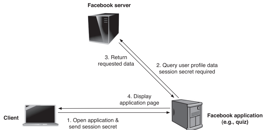
Fig. 1. Data-flow in Facebook.
