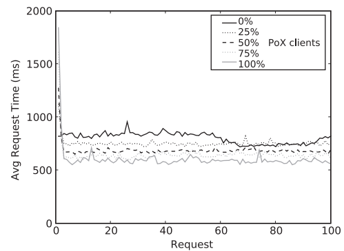
Fig. 6. Data request time comparison for mixed PoX and original API clients.
