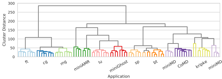
Fig. 2: Clustering of 11 applications, with two different input configurations running on 4 nodes each. The colors are assigned manually to represent different applications.
